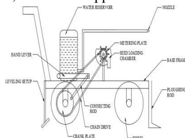
Fig.1: 2D Model of the machine
