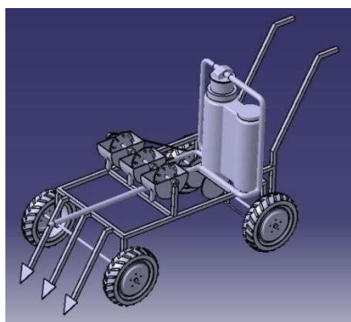
Fig.2: 3D Model of the machine
