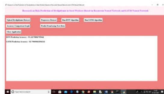
Figure.8: LSTM algorithm
