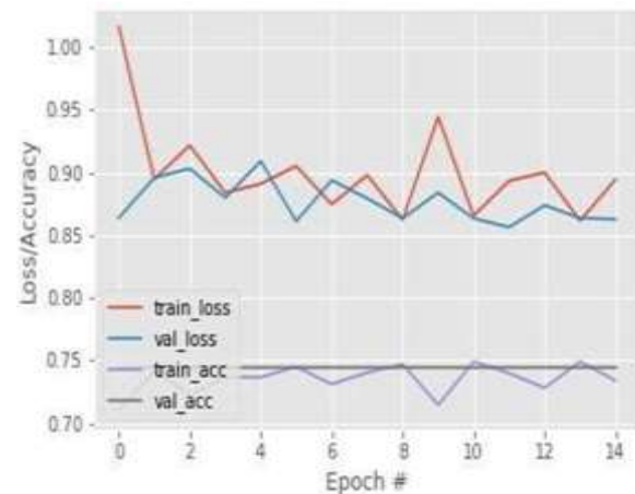
Fig -6: Plot between loss and epoch
